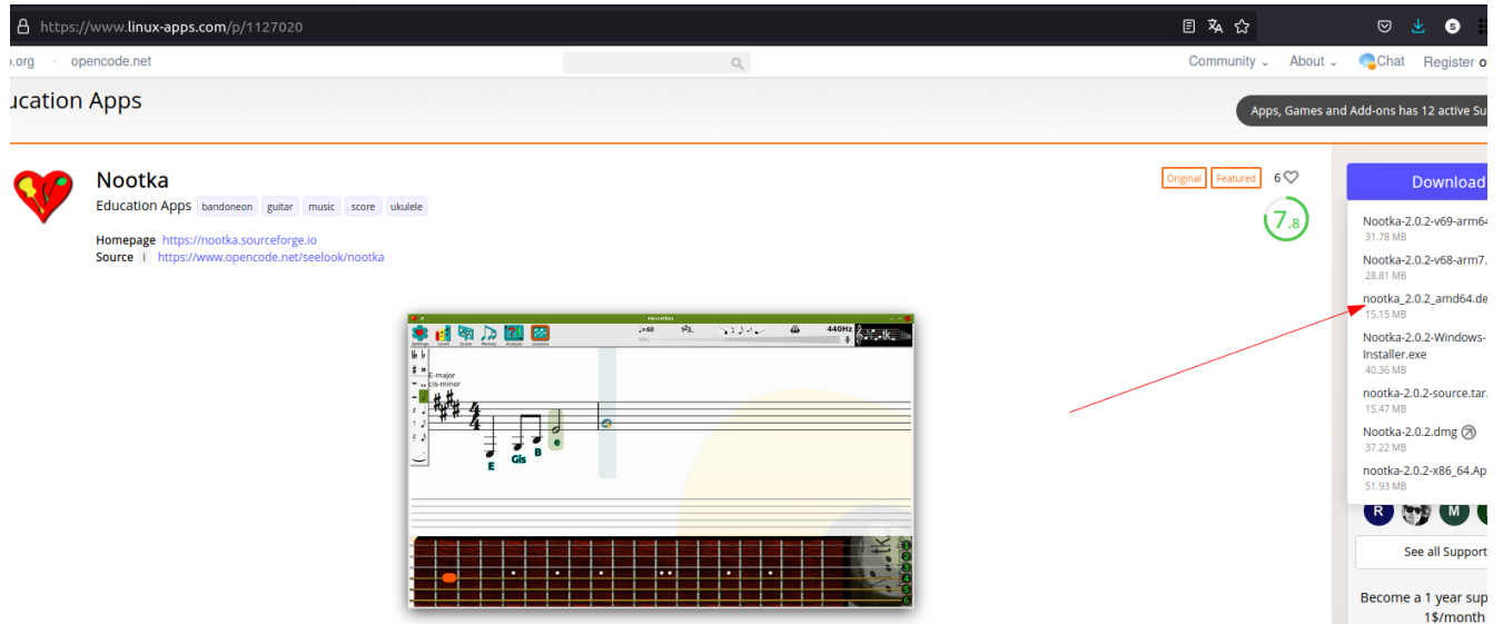
image 6.5.3 - Descargando Software
